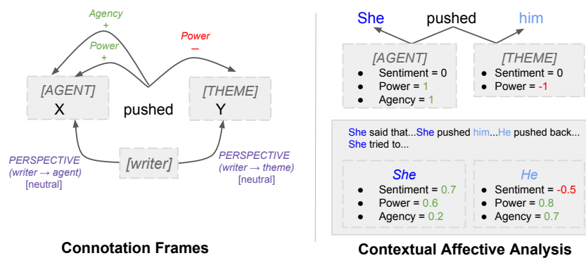
Figure 2.1: Left, we show off-the-shelf connotation frame annotations (Rashkin et al., 2016; Sap et al., 2017) for the verb “push”. Right, we show the proposed adaptation. We adapt connotation frames from a verb-centric formalism to an entity-centric formalism, transferring scores from verbs to entities using a context-aware approach (top right). We then aggregate contextualized scores over all mentions of entities in a corpus (bottom right). This new approach— contextual affective analysis —enables us to obtain sentiment, power, and agency scores for entities in unannotated corpora and conduct extensive analyses of people portrayals in narratives, which we exemplify on #MeToo data.
