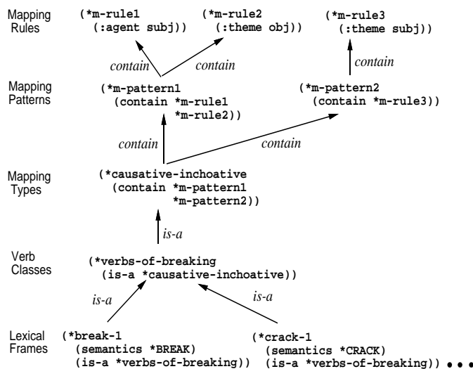
Figure 1: Lexical Hierarchy Example: English
