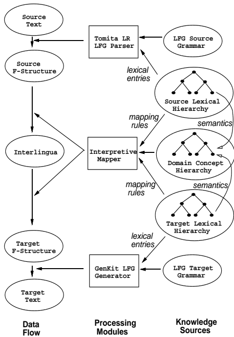
Figure 3: Architecture for Machine Translation
