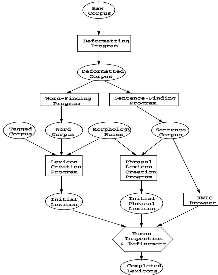
Figure 3: Automation of Source Lexicon Acquisition
