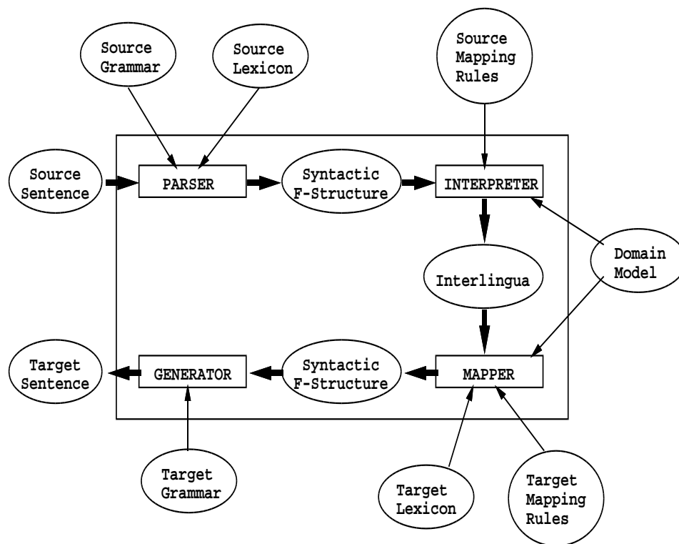
Figure 1: The Run-Time Architecture of KANT
