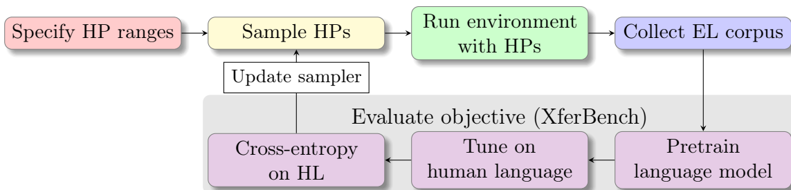
Figure 5.2: Illustration of hyperparameter optimization with XferBench.
