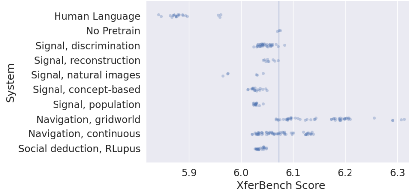
Figure 3.2: XferBench score across ELCC and human language baselines; lower is better. “No pretrain” baseline illustrated with the line on the plot.
