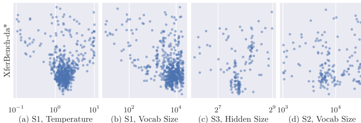
Figure 5.3: Examples of different hyperparameter–objective relations observed in the various searches and hyperparameters. From left-to-right, we have: (a) a clear best value, (b) a clear trend outside the provided range, (c) a weak trend toward a particular value, and (d) no definite trend. The y -axis based on different “sizes” of XferBench-da normalized to similar scales.
