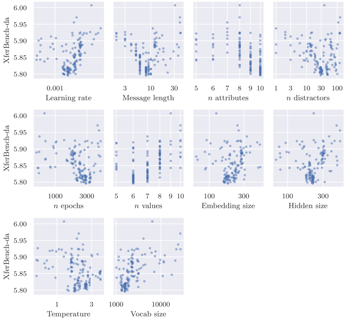
Figure D.4: Objective values for Search 3 by individual hyperparameter.
