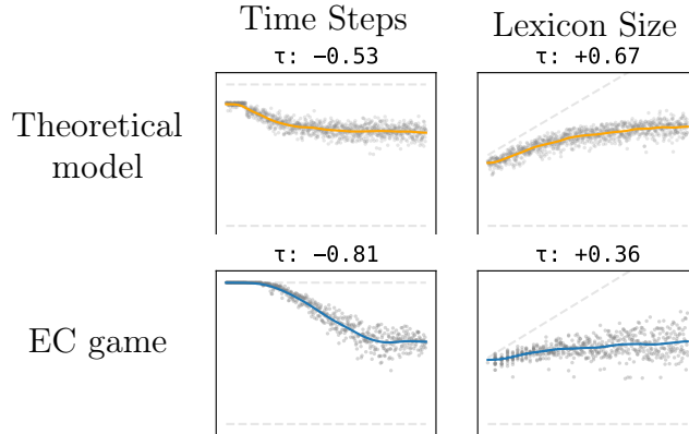
Figure 2.3: Plots of lexicon entropy ( y -axis) versus time steps and lexicon size ( x -axes) comparing a theoretical model against empirical measurements on navigation game with emergent communication (from Boldt et al. (2022b)). 8 Theoretical models can help predict the outcomes of emergent communication games much more efficiently than simply running the environment while also providing a conceptual understanding the environment’s behavior.
