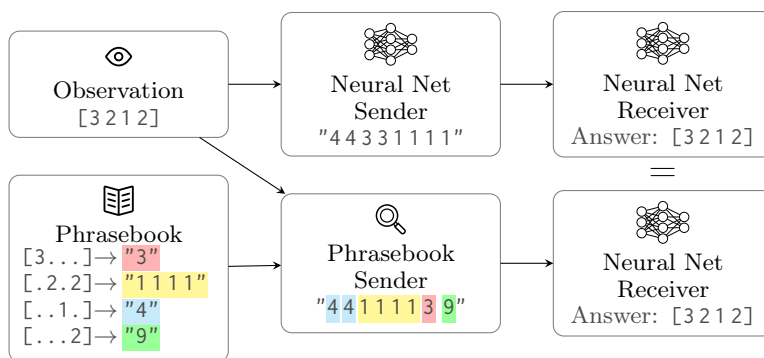
Figure 7.1: Main experimental setting where we compare a phrasebook-based agent with the original neural network-based sender. We also experiment with a phrasebook-based receiver.
