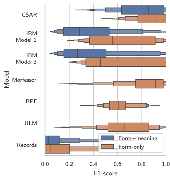
Figure E.1: Exact F_1 scores of baseline methods on the procedural datasets
