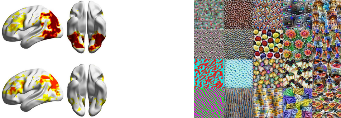
(a) Visualization of fMRI scans of the human brain in response to visual stimuli (Bracci et al., 2023).
