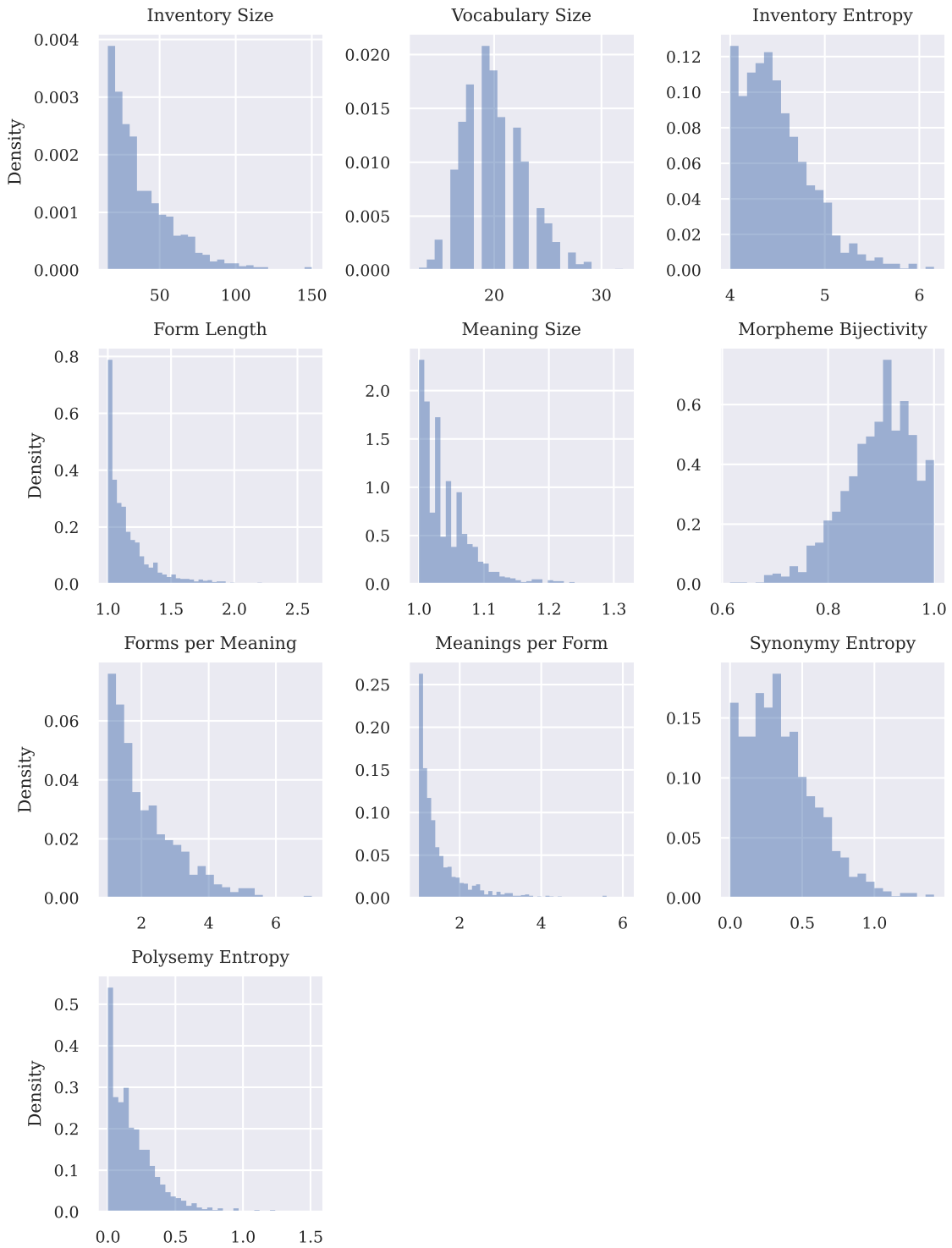
Figure F.1: Histograms of metrics from main experiment.
