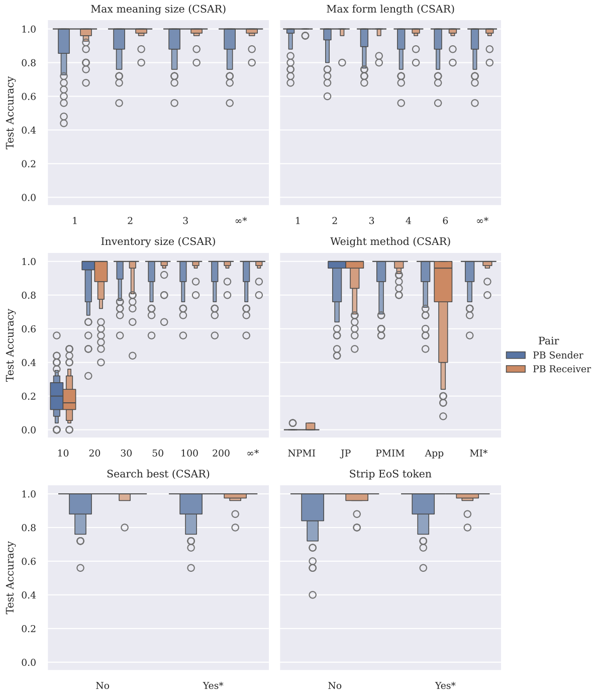
Figure F.5: Phrasebook agents’ test accuracy across morpheme induction and phrasebook agent ablations. *Default values.
