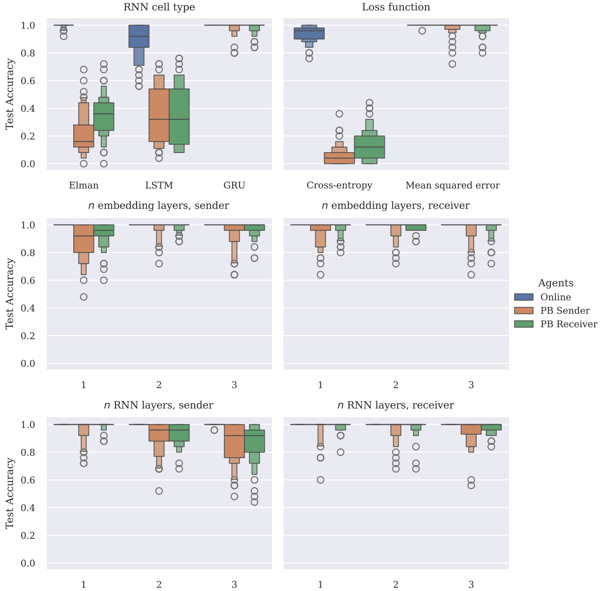
Figure F.4: Phrasebook agents' test accuracy across morpheme induction and phrasebook agent ablations. *Default values.
