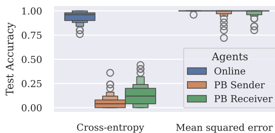
Figure 7.3: Accuracy plot for loss function ablation experiment. Full plots in Appendix F.6.
