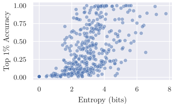
Figure D.1: Entropy versus accuracy for Search 5r.
