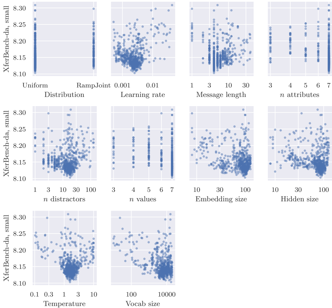
Figure D.2: Objective values for Search 1 by individual hyperparameter.
