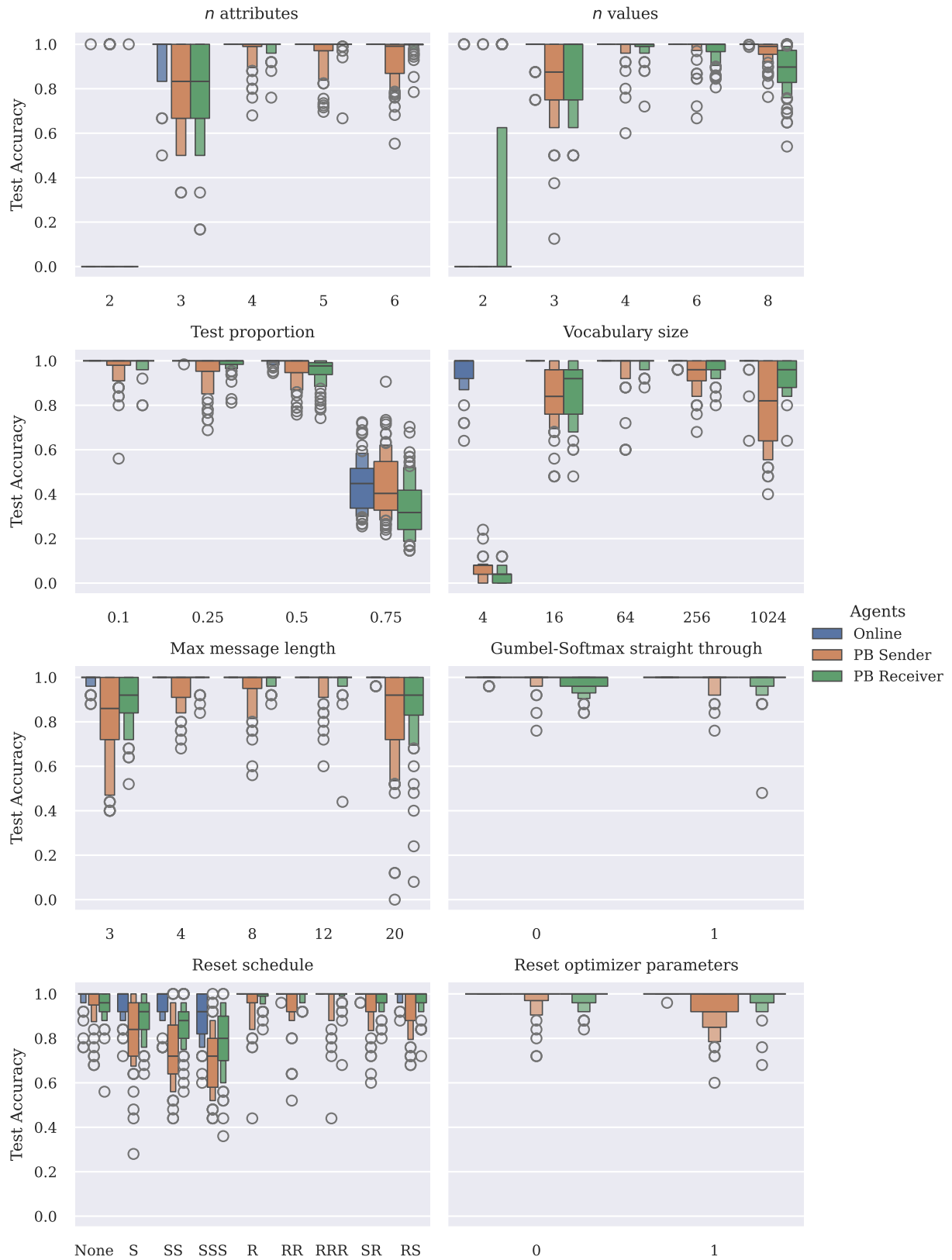
Figure F.3: Phrasebook agents' test accuracy across morpheme induction and phrasebook agent ablations. *Default values.
