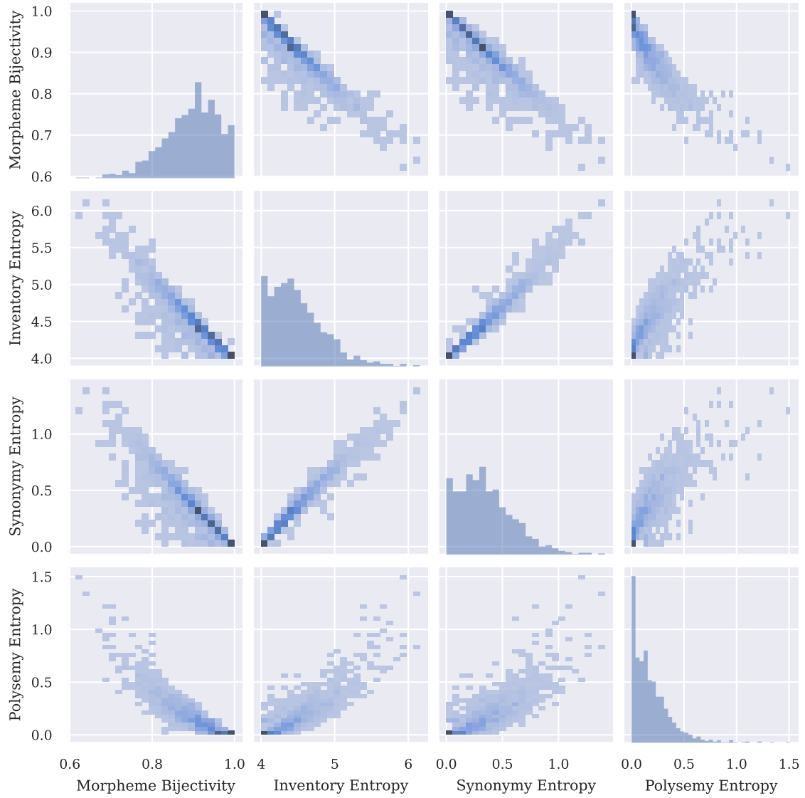
Figure F.2: Bivariate histograms of selection of metrics from main experiment.
