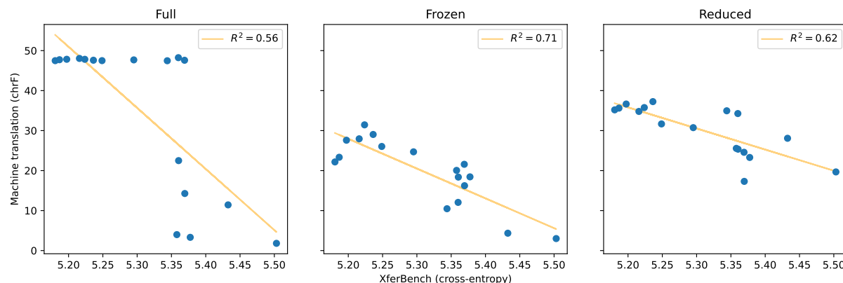
Figure C.1: Scatter plots showing XferBench score versus machine translation score.
