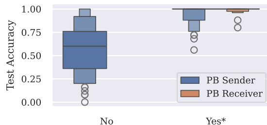
Figure 7.4: Accuracy plots various for repeat morpheme phrasebook sender ablation. Full plots in Appendix F.7.
