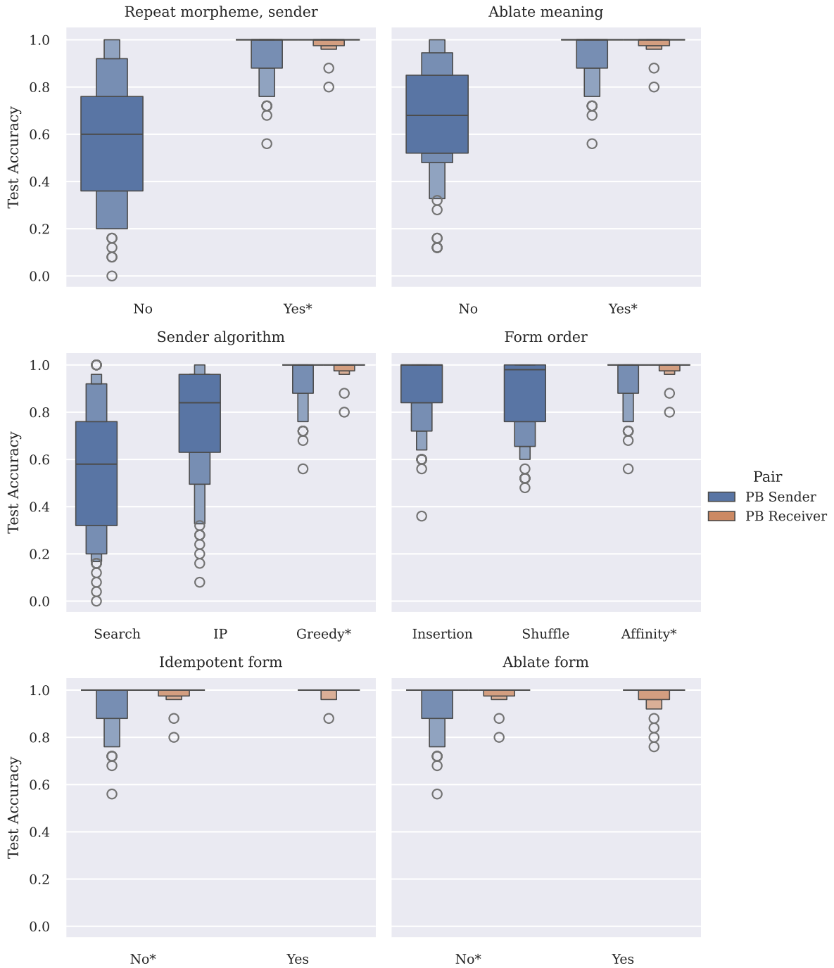
Figure F.6: Phrasebook agents' test accuracy across morpheme induction and phrasebook agent ablations. *Default values.
