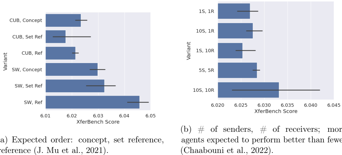
Figure 3.5: XferBench scores compared to expected order; lower is better.
