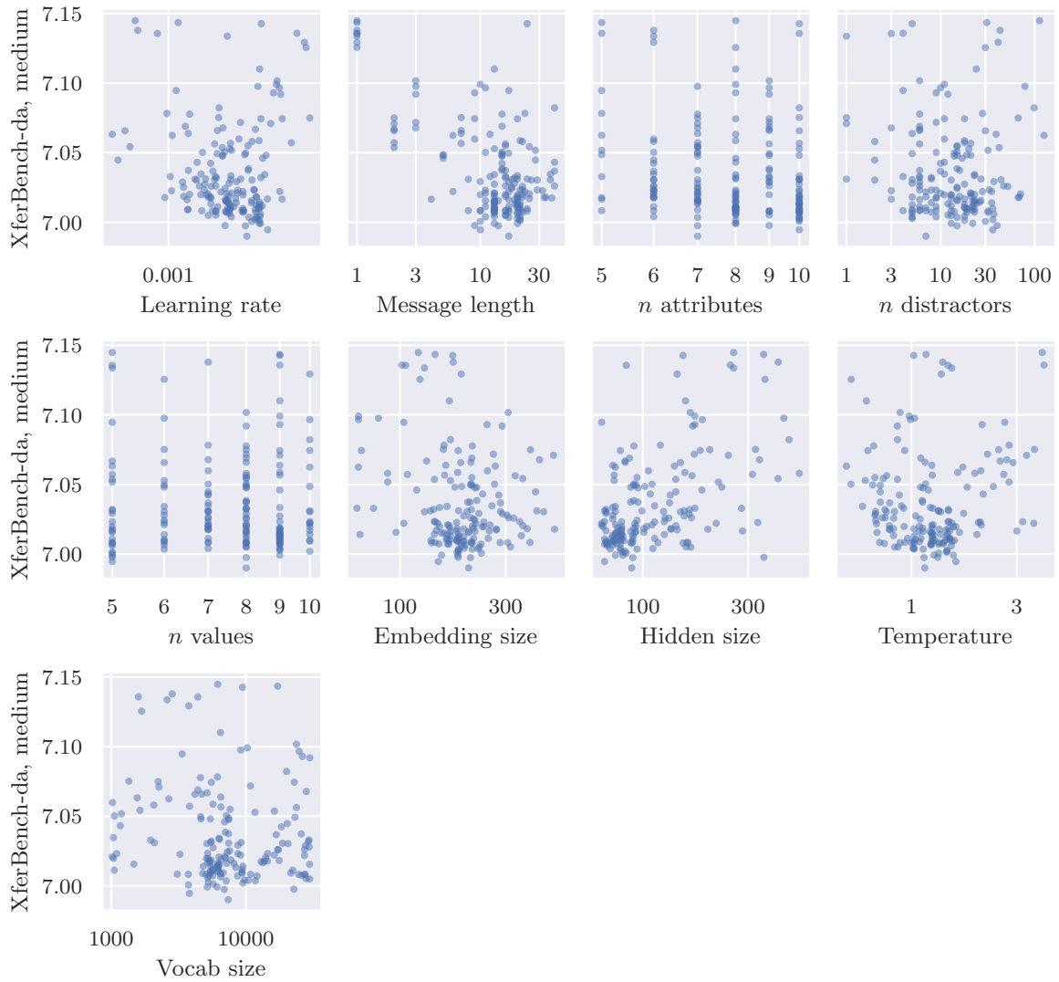
Figure D.3: Objective values for Search 2 by individual hyperparameter.
