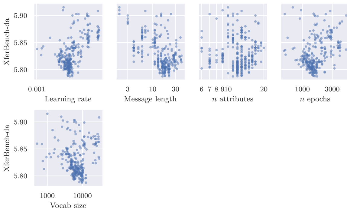
Figure D.5: Objective values for Search 4 by individual hyperparameter.
